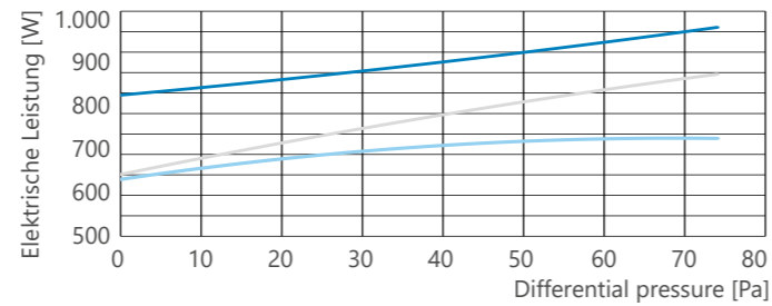
Electrical power vs. Differential pressure
