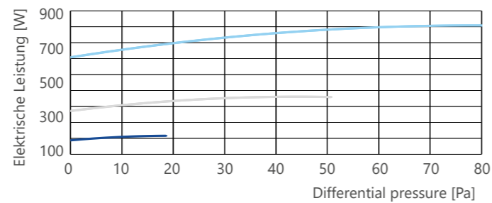
Electrical power vs. Differential pressure
